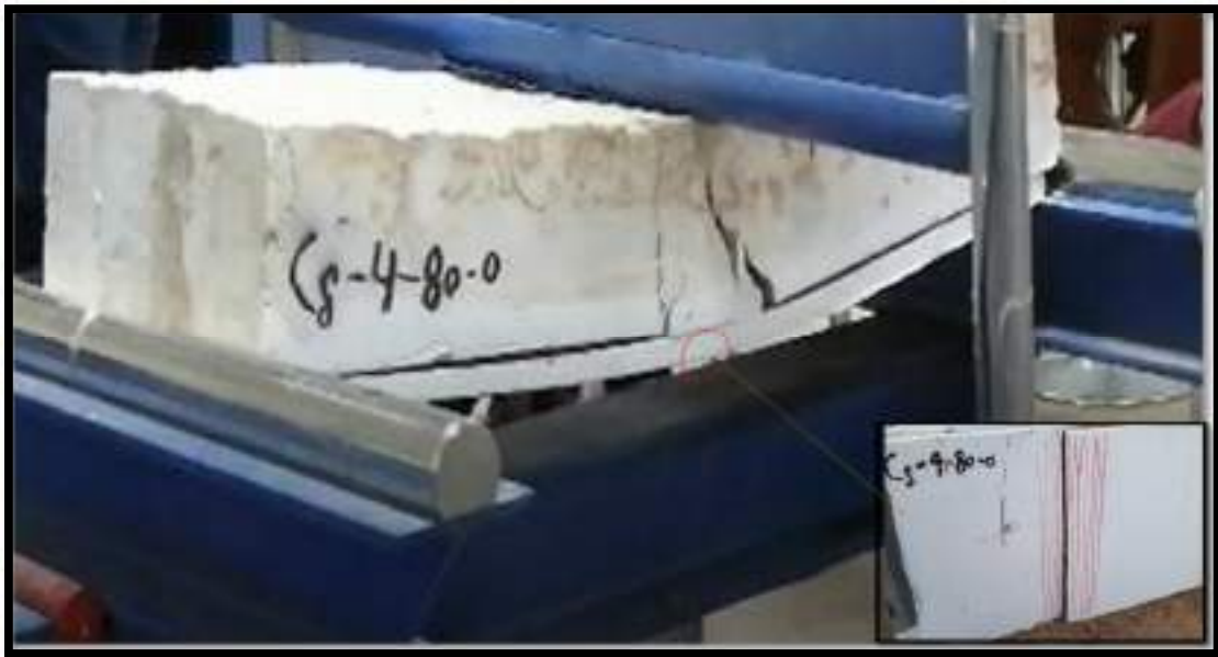
(c) Mode of failure for Cs-4-80-0 specimen.
