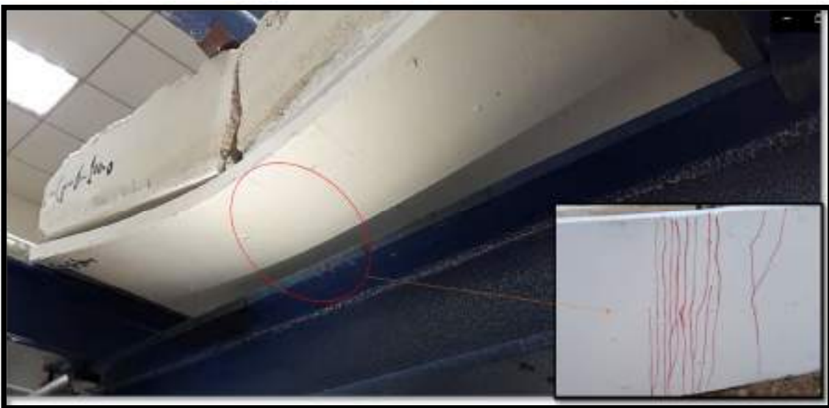
(f) Mode of failure for Cs-6-100-0 specimen.
