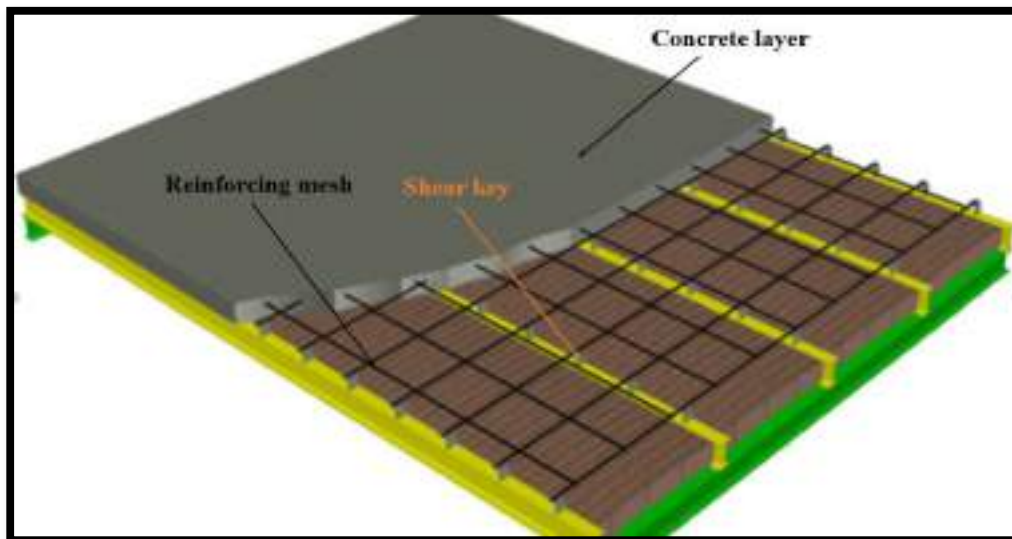
Figure 2-3: Retrofitting jack-arch slab by concrete layer method [16].
