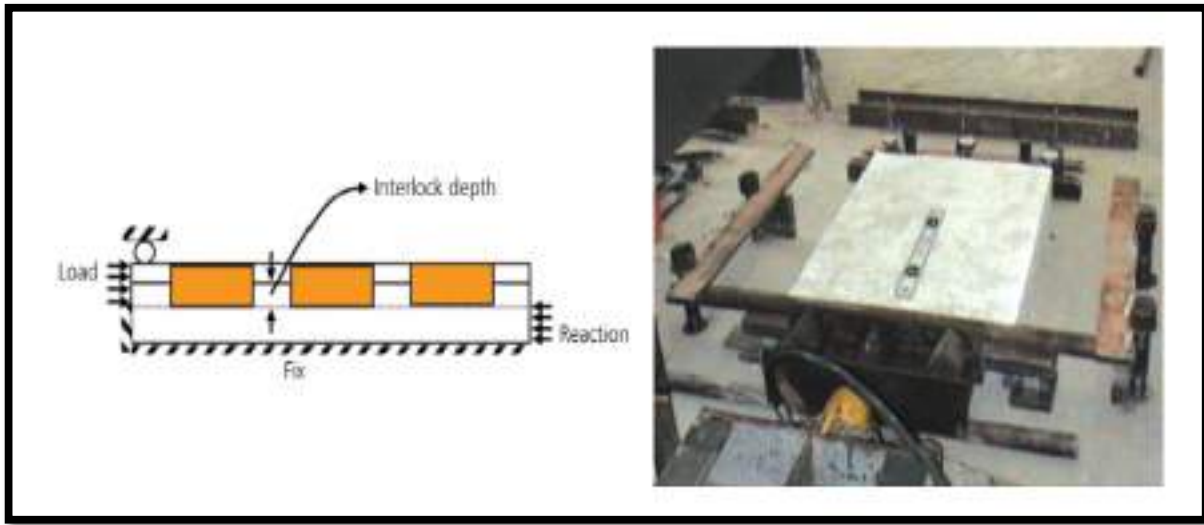
Figure. 2-23: Pure shear loading test for slab specimens [30].
