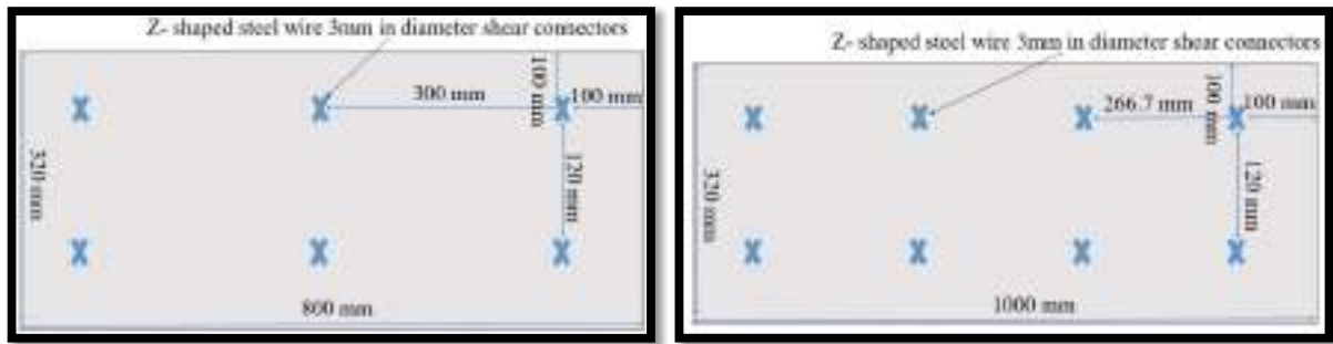
(a) Specimen span (800) mm.
