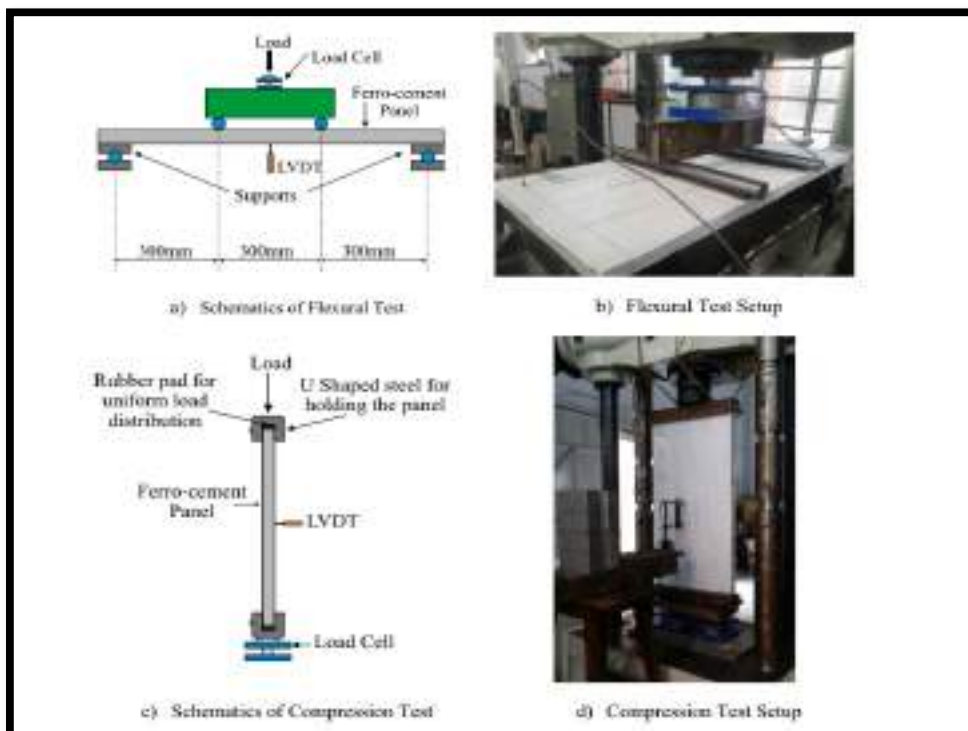
Figure 2-17: Test setups.
