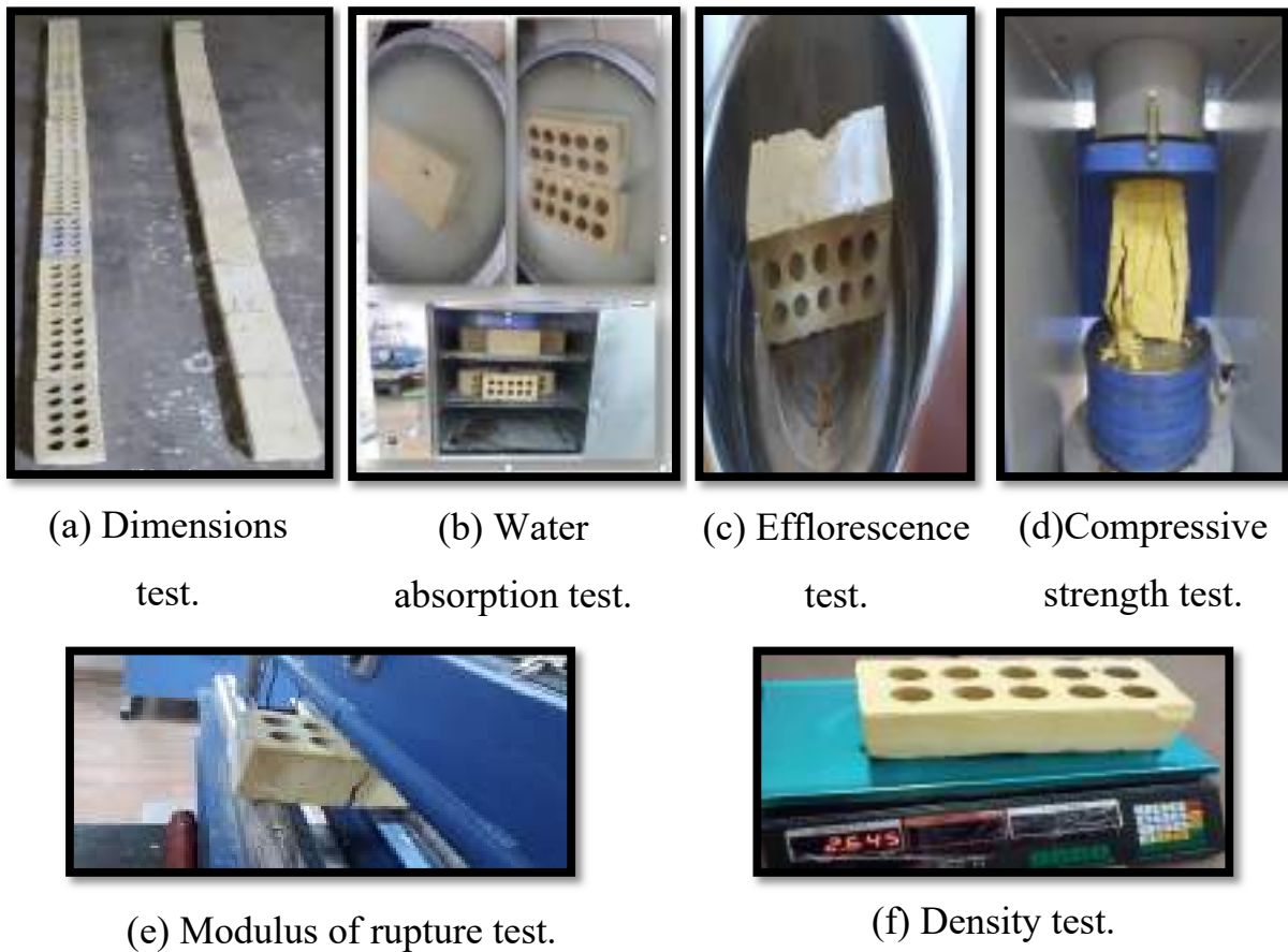
Figure 3-1: Clay bricks test.
