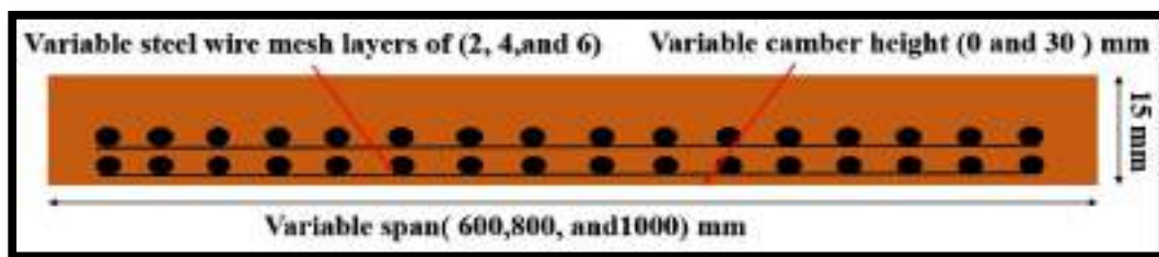
(a) Precast ferrocement layers.
