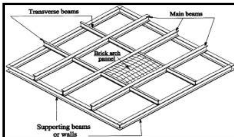
Figure. 2-1: Details of a of the proposed two-way arch slab [5].
