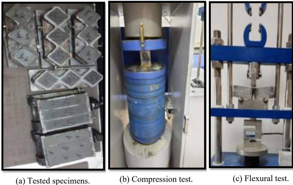
Figure. 3-11: Samples testing of trail mix mortar.
