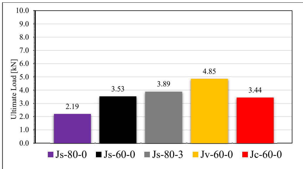
Figure 4-1: Ultimate loads results for jack arch control specimens G_1 .
