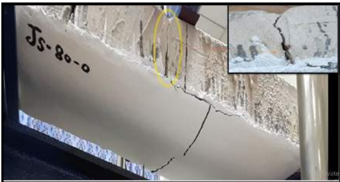
(b) Mode of failure for Js-80-0 specimen.
