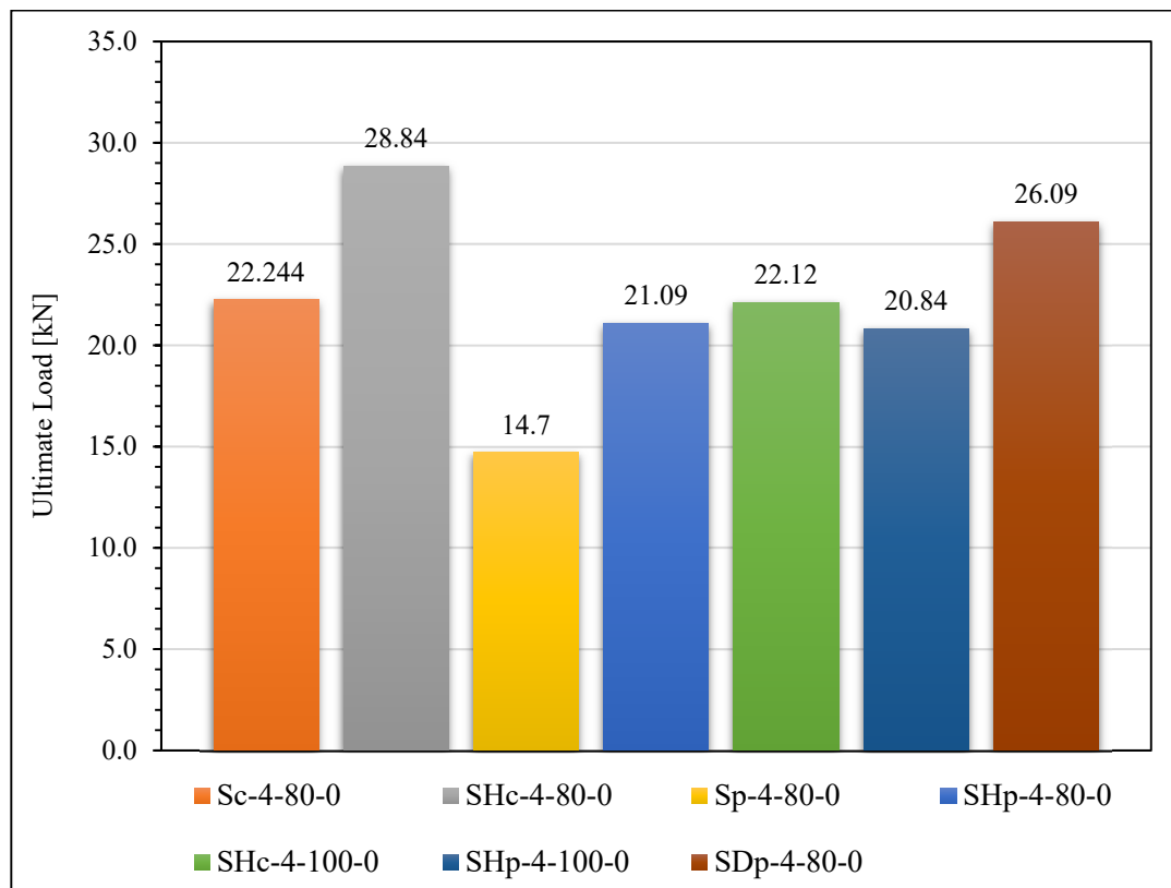
Figure 4-3: Ultimate strength loads results for ferrocement sandwiched slabs specimens G 3 .
