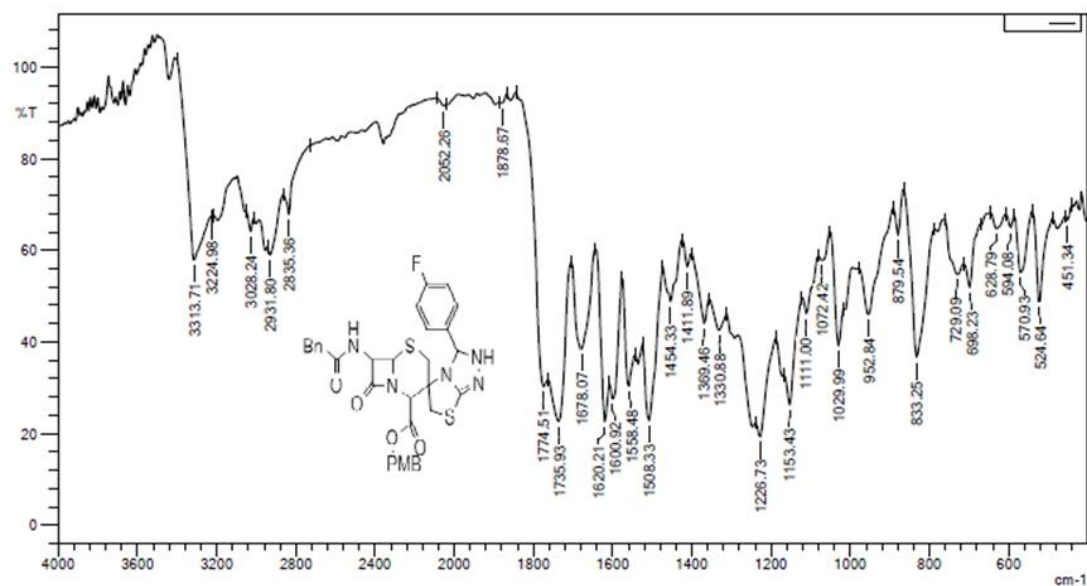
Fig (3-41) IR Spectrum of the compound B5
