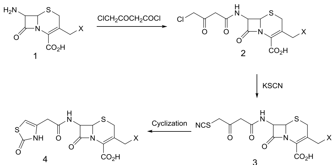
Scheme 1-3: Synthesis of 7-oxothiazolinyl cephalosporins
