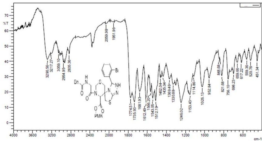
Fig (3-34) IR Spectrum of the compound B3
