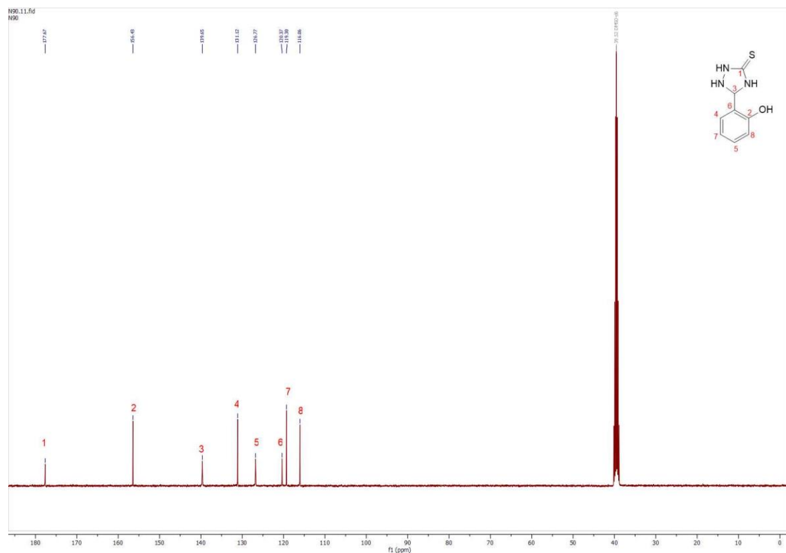
Fig (3-12) 13 C NMR Spectrum of the compound A4
