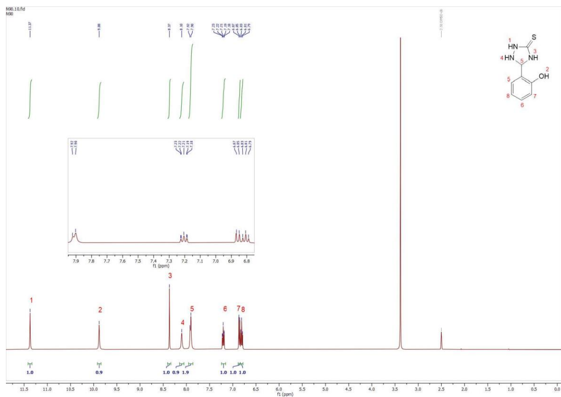
Fig (3-11) 1 H NMR Spectrum of the compound A4
