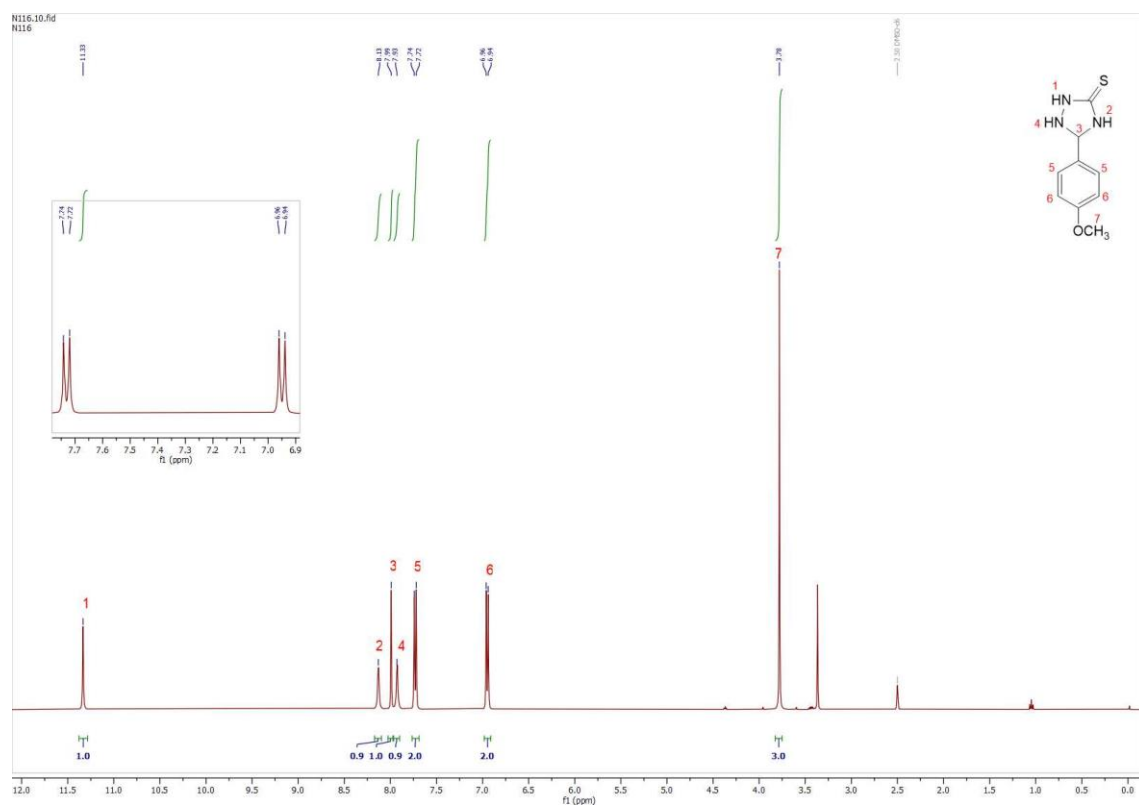
Fig (3-26) ^1\text{H} NMR Spectrum of the compound A9
