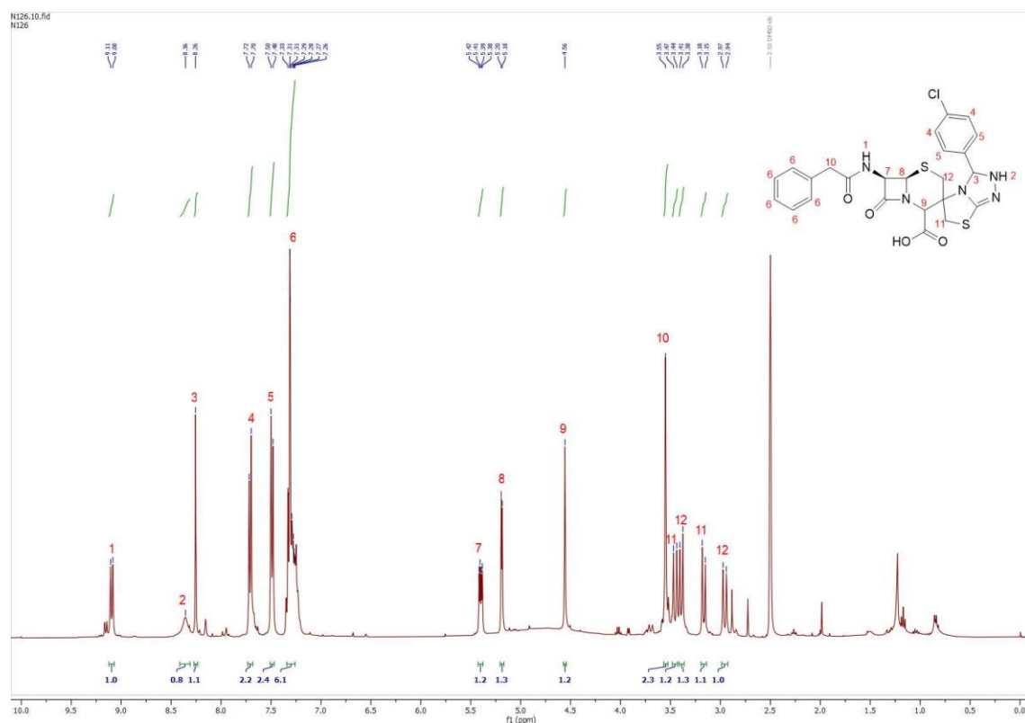
Fig (3-72) ^1\text{H} NMR Spectrum of the compound C6
