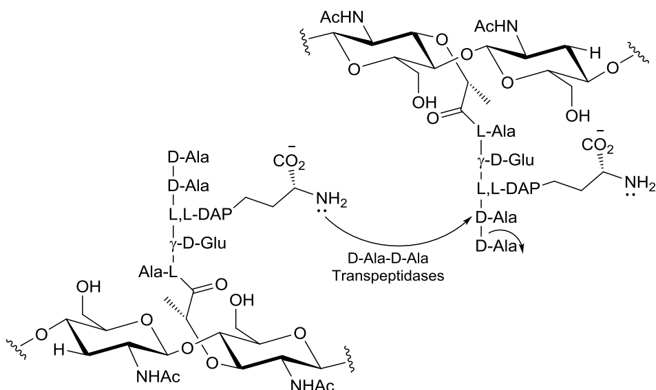
Scheme 1-1: Cross linkage by D-Ala-D-Ala transpeptidases in E.coli
