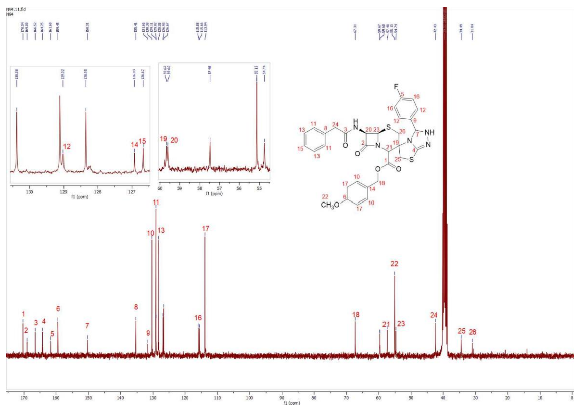
Fig (3-43) ^{13}\text{C} NMR Spectrum of the compound B5
