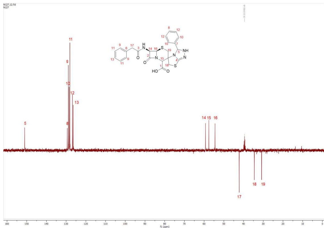
Fig (3-53) DEPT 135 Spectrum of the compound C1
