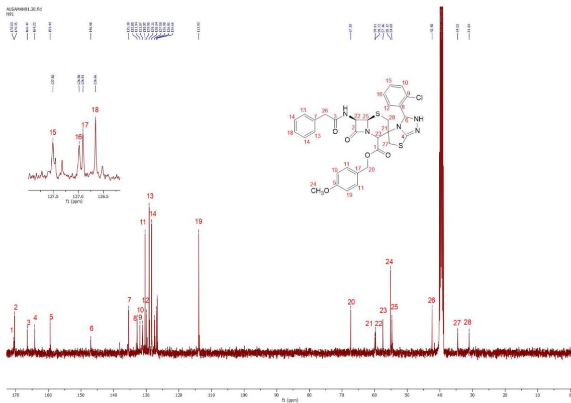
Fig (3-33) ^{13}\text{C} NMR Spectrum of the compound B2
