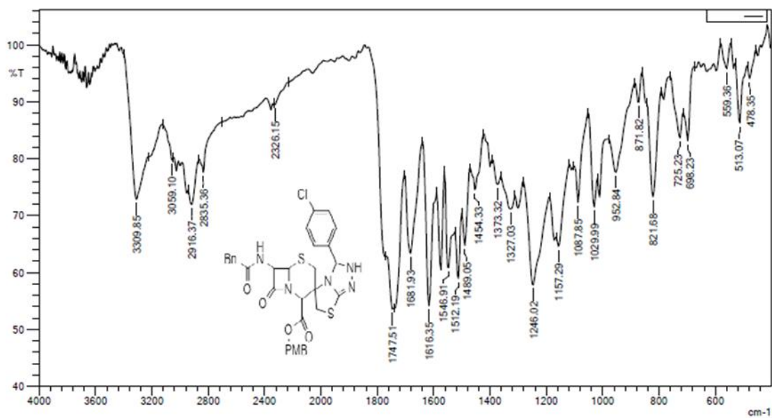
Fig (3-44) IR Spectrum of the compound B6
