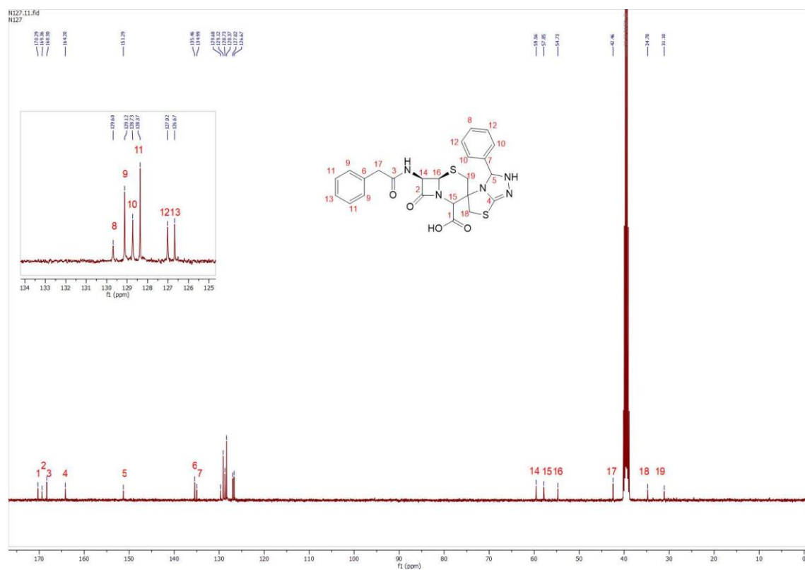
Fig (3-52) ^{13}\text{C} NMR Spectrum of the compound C1
