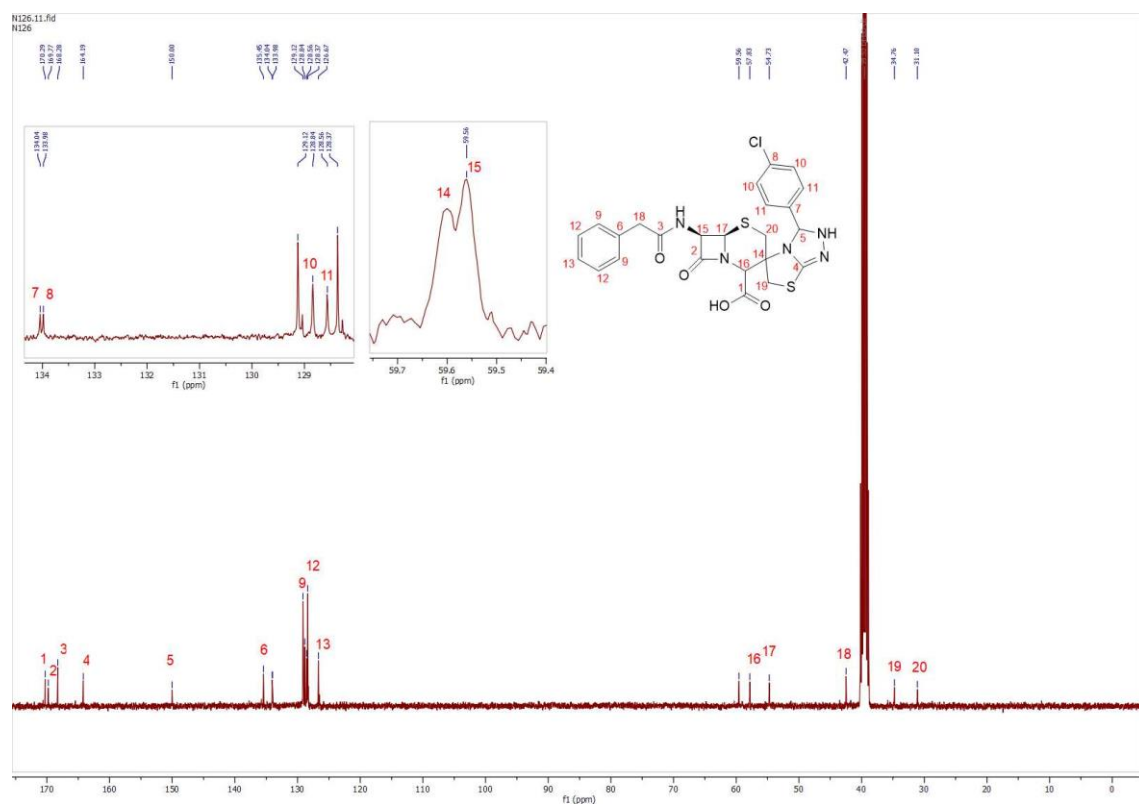
Fig (3-73) ^{13}\text{C} NMR Spectrum of the compound C6
