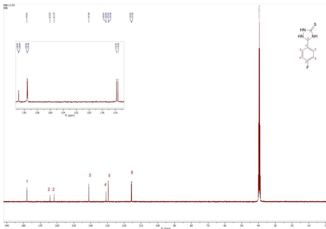
Fig (3-15) 13 CNMR Spectrum of the compound A5
