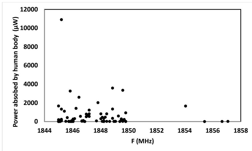
Fig. 5c. The values of power density absorbed by the human body at 1845 MHz
