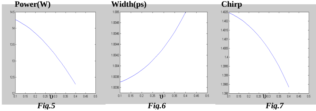
Fig. (5,6and7).The power P , width and chirp of soliton as a function of different values of v respectively .
