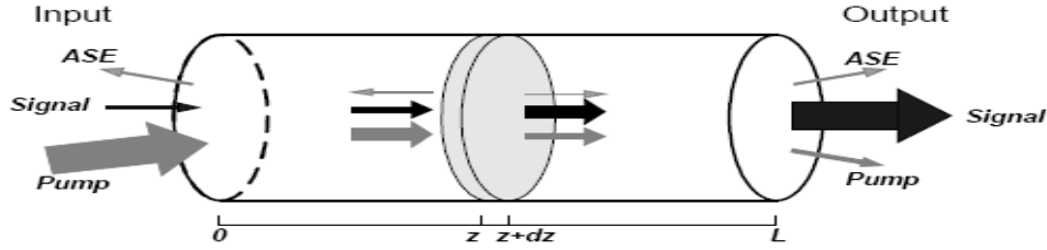
Fig. 2 Basic EDFL Operation
