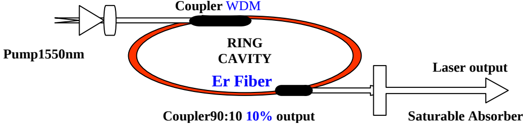
Fig. (3) schematic diagram for theoretical model WDM, wavelength division multiplexer.
