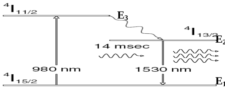
Fig. 1 Energy-levels of Erbium in Silica Glass
