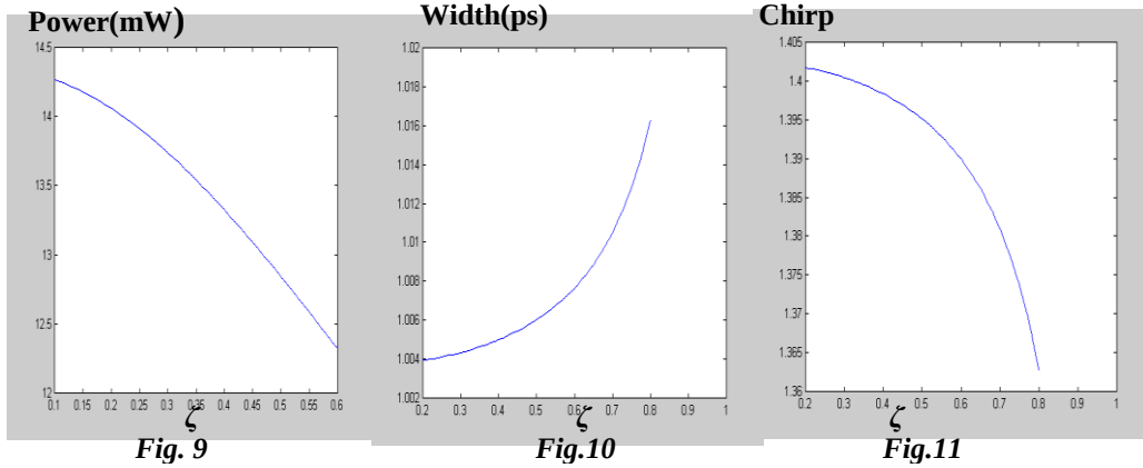
Fig. (9,10and11).The power P , width and chirp of soliton as a function of different values of \zeta respectively .
