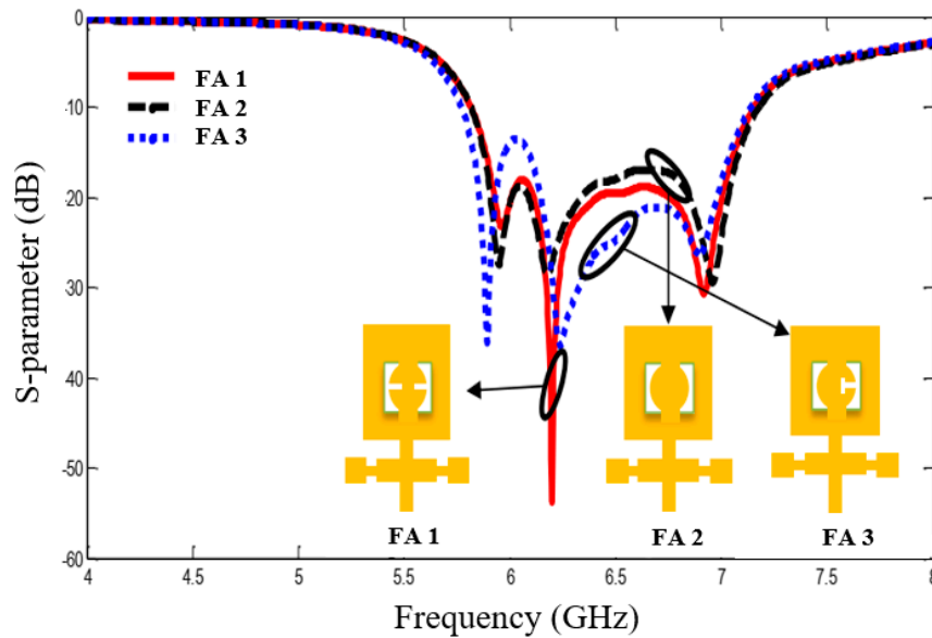
Figure 5. S11-parameter of the proposed filtering antenna (FA) for different shaped slots.
