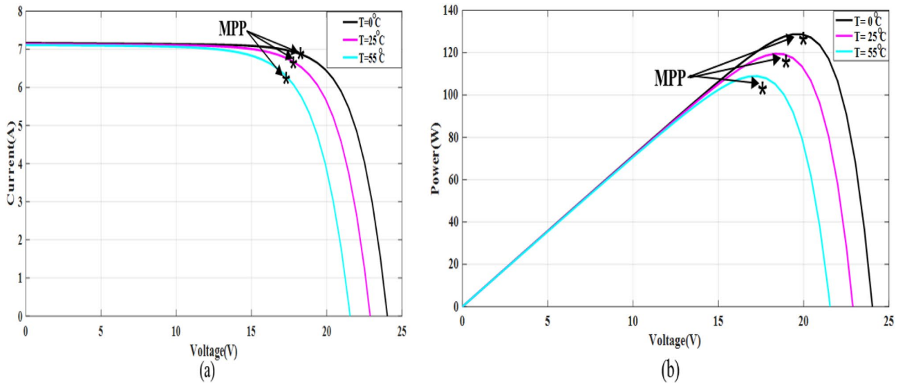
Figure 12. I-V and P-V graphs of double-diode model at different values of temperature and fixed irradiation, G = 1000 \text{ W/m}^2 (a) I-V graph and (b) P-V graph.
