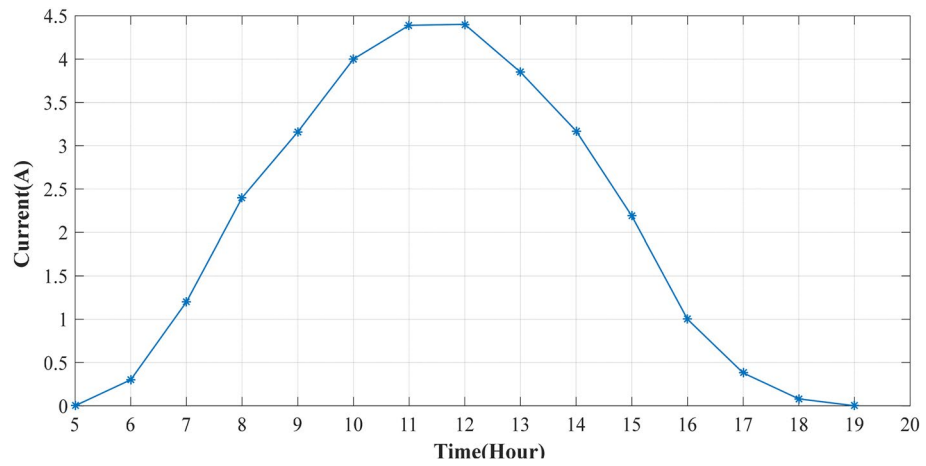
Figure 18. Experimental current of the NST-PV module.
