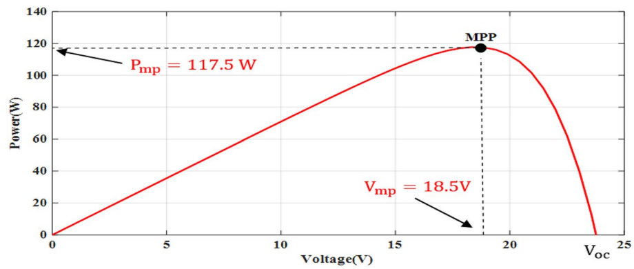
Figure 9. P-V graph of single-diode model at STC.
