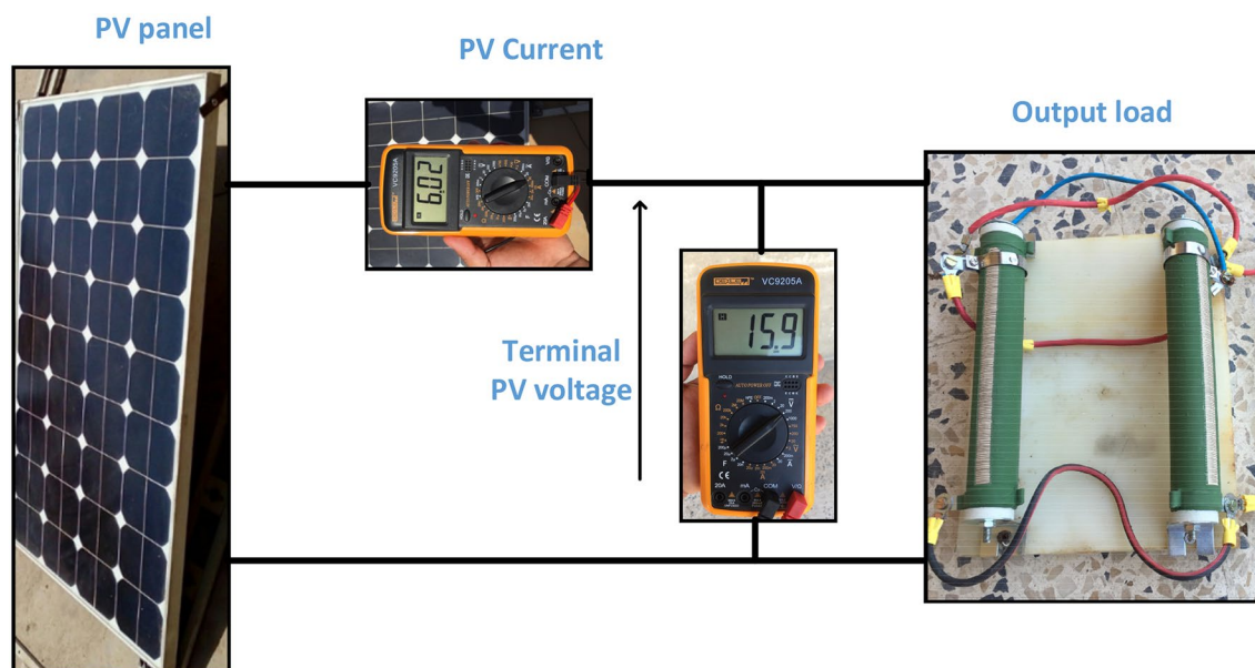
Figure 14. Experimental components of the proposed PV system.
