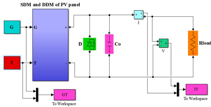
Figure 4. Simulink/Matlab block diagram of the NST-120 PV panel.
