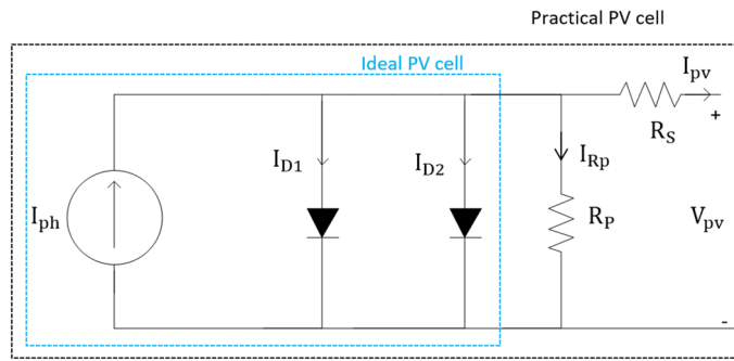
Figure 2. Double-diode PV model circuit.
