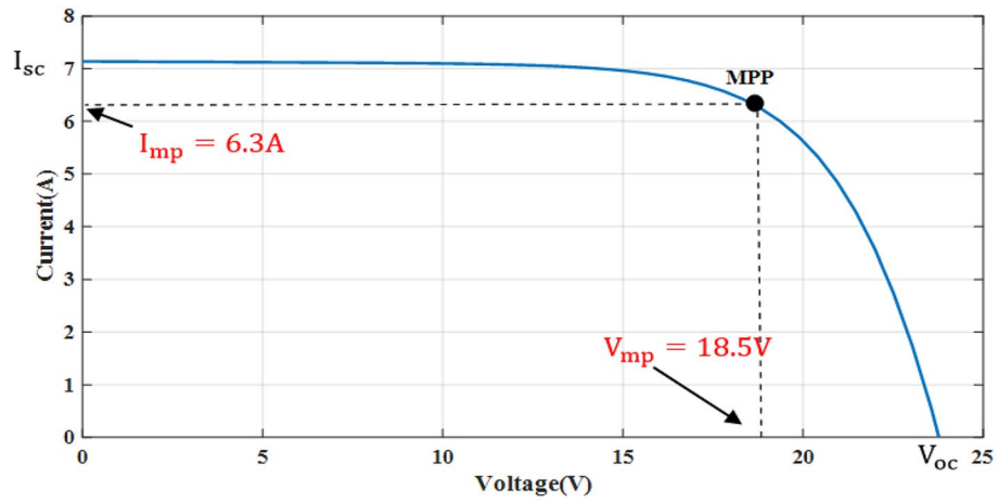
Figure 8. I-V graph of single-diode model at STC.
