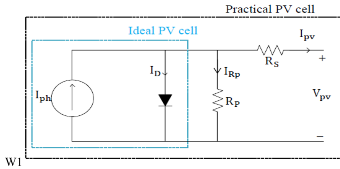
Figure 1. Single-diode model of the PV cell.
