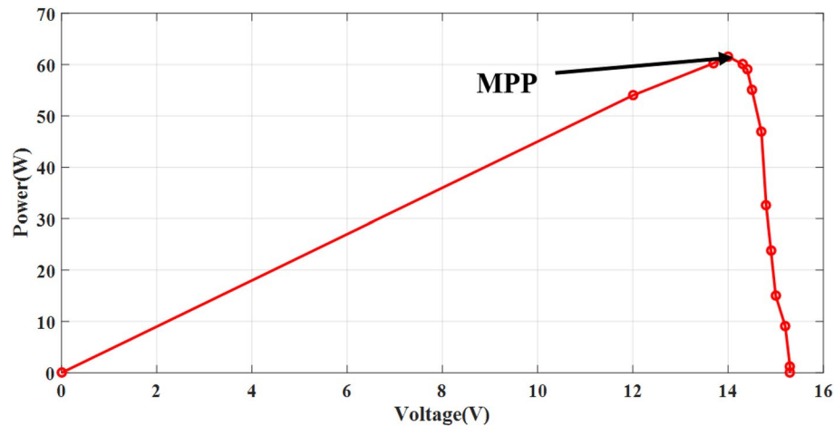
Figure 21. Experimental P - V graph of the NST PV module.
