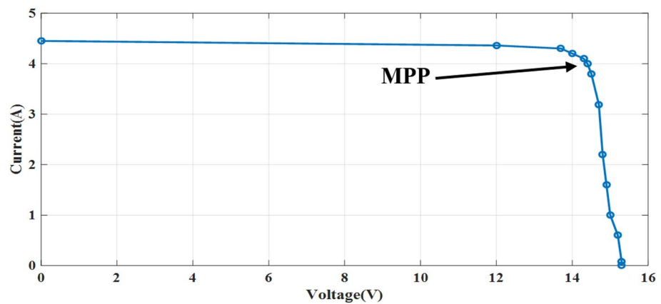
Figure 20. Experimental I - V graph of the NST PV module.
