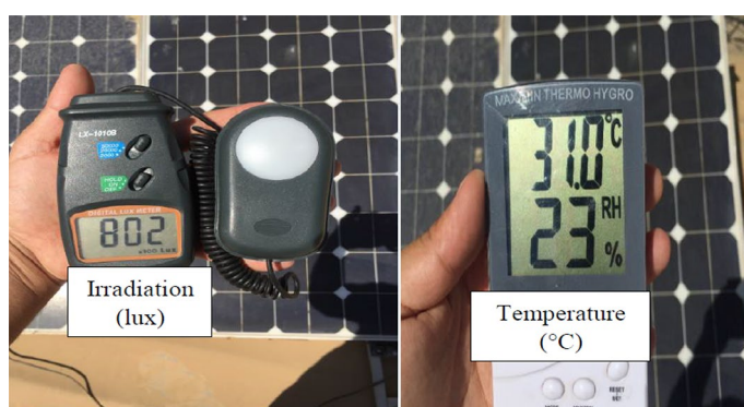
Figure 16. Measurements of irradiance and temperature for the proposed PV system.
