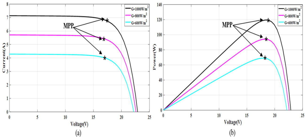
Figure 13. I-V and P-V graphs of double-diode model under different values of irradiation and constant temperature, T = 25 \text{ }^\circ\text{C} (a) I-V graph and (b) P-V graph.
