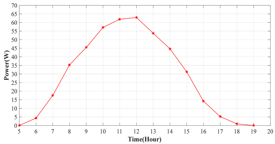
Figure 19. Experimental power of the NST PV module.
