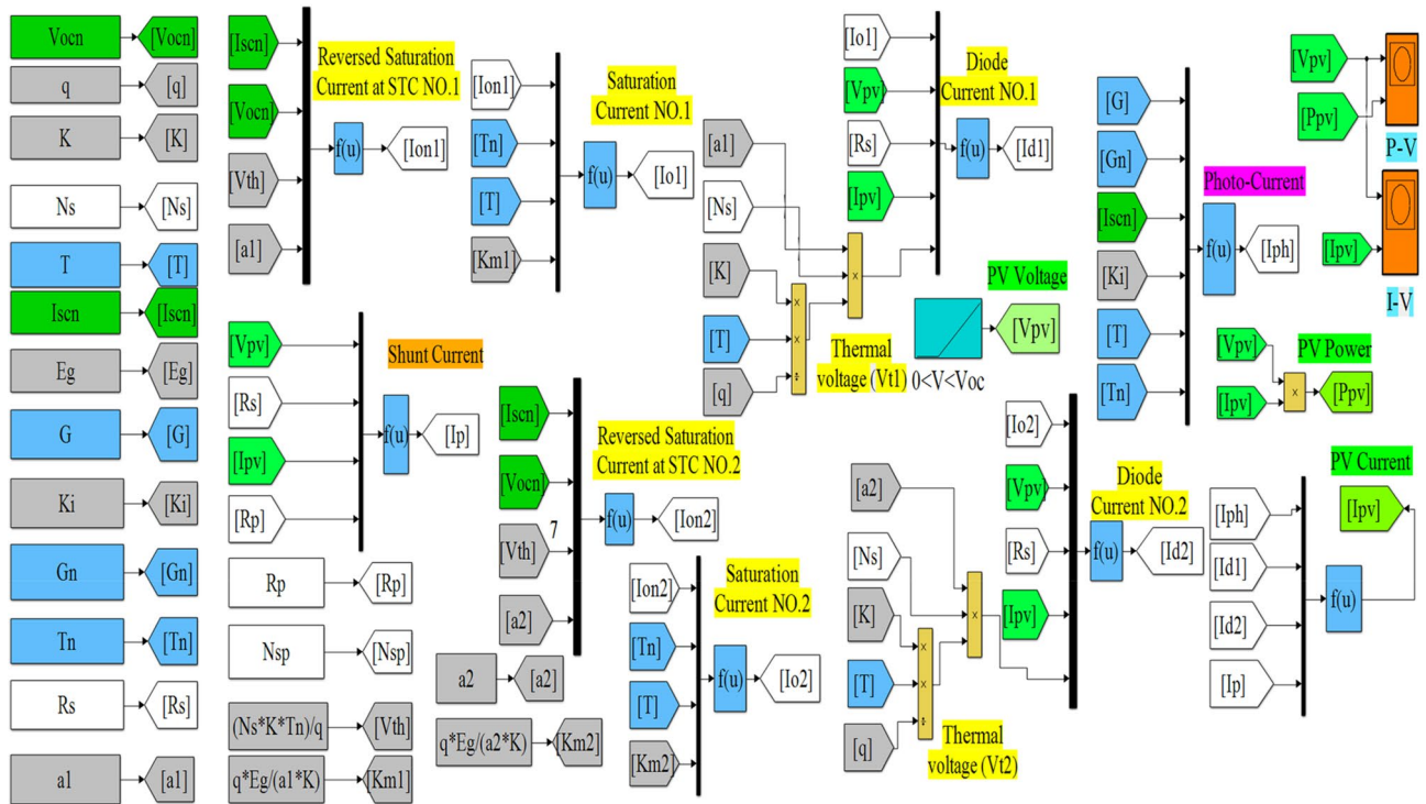
Figure 6. Double-diode model in Matlab.
