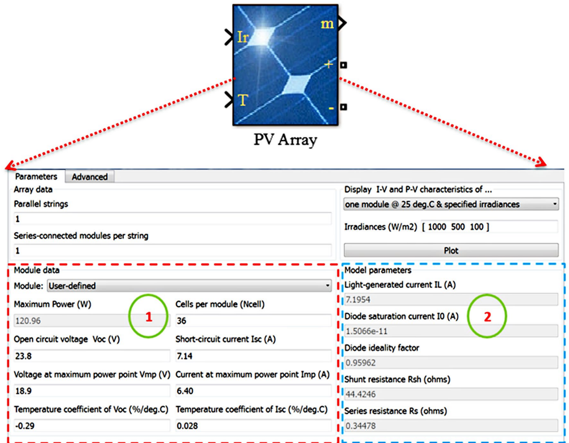
Figure 3. Extracted parameters of the NST-120 panel.
