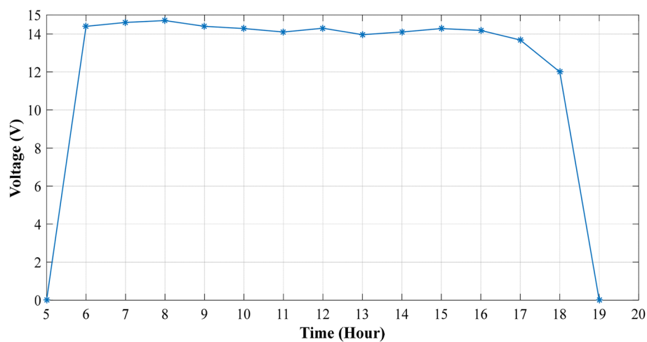
Figure 17. Experimental voltage of the NST-PV panel.
