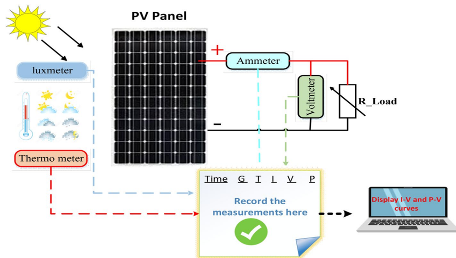
Figure 7. Proposed PV system components.
