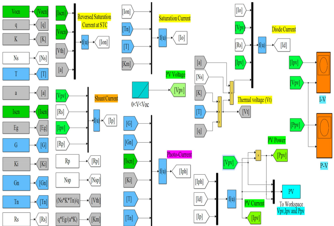
Figure 5. Single-diode model in Matlab.
