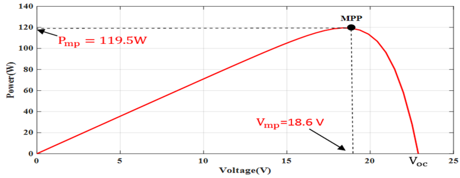
Figure 11. P-V graph of double-diode PV model at STC.
