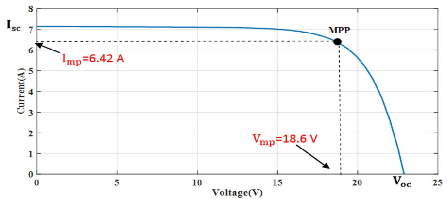
Figure 10. I-V graph of double-diode model at STC.
