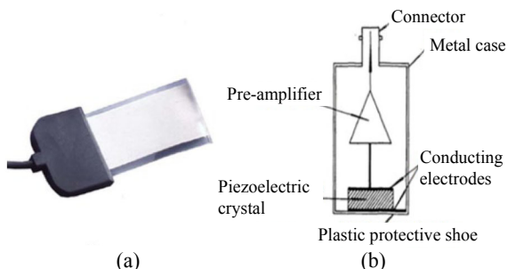
Fig. 4 Acoustic sensors: (a) piezoelectric film sensor with its connector and (b) typical design of the piezoelectric transducer sensor [22].
