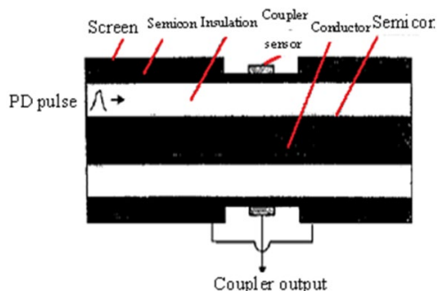
Fig. 3 Diagram of a capacitive coupler [21].
