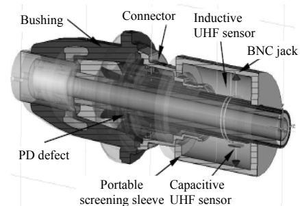
Fig. 7 Plug-in cable termination and principle of the UHF PD diagnostics [1].
