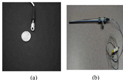
Fig. 6 Optical sensors (extrinsic): (a) extrinsic Fabry-Perot interferometer sensor [25] and (b) extrinsic microelectromechanical system sensor [25].
