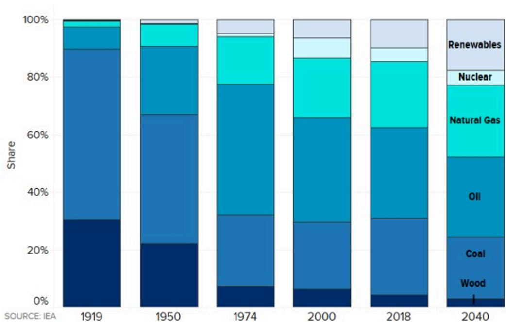
Fig. 4. Global energy dependency from 1919 to 2040 (IEA, 2019)
