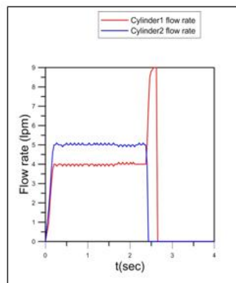
Fig .(6-b) cylinders inlet flow rate without flow divider valve
