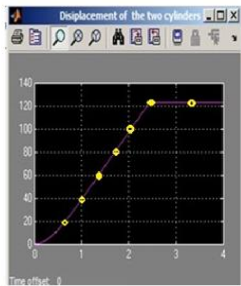
Fig .(5-a) cylinders displacement with flow divider valve.
