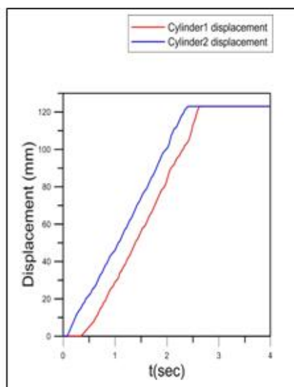
Fig . (6-a) cylinders displacement without flow divider valve.
