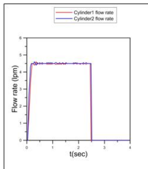
Fig .(8-b) cylinders inlet flow rate with flow divider valve at 45 °c
