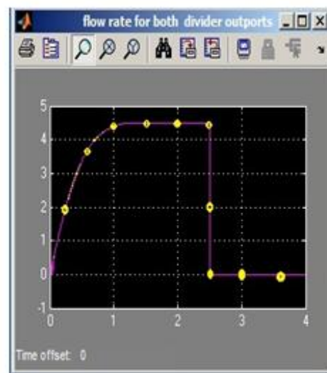
Fig .(5-b) cylinders inlet flow rate with flow divider valve.
